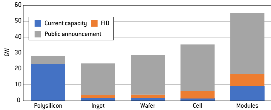
Figure 2: Solar manufacturing expansion in Europe up to 2026
